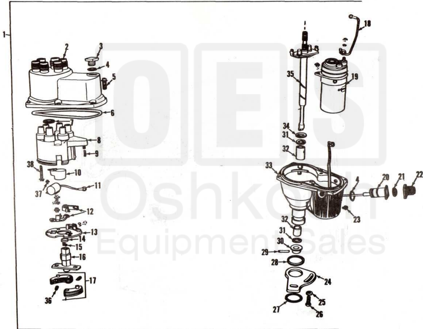
Figure 21. Distributor.
